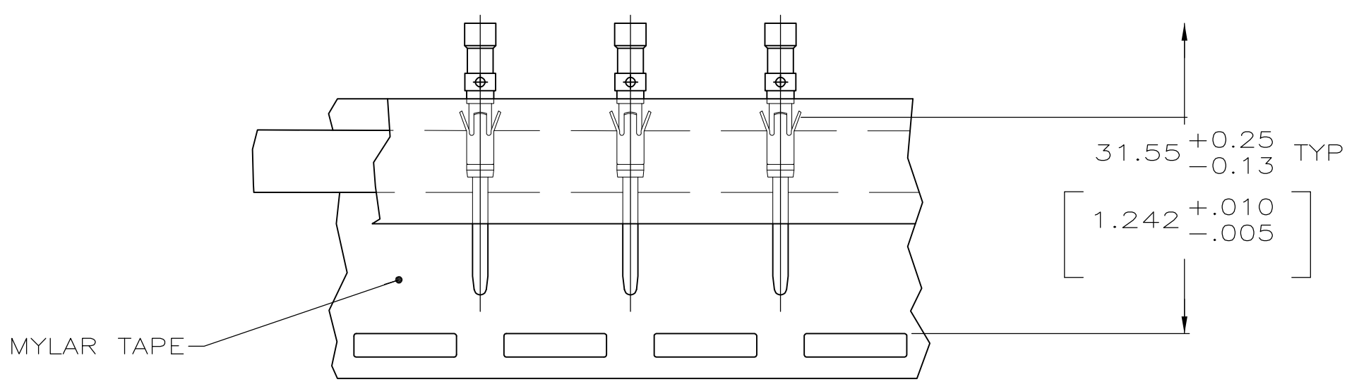
TAPE MTG DETAIL SCALE 2:1
