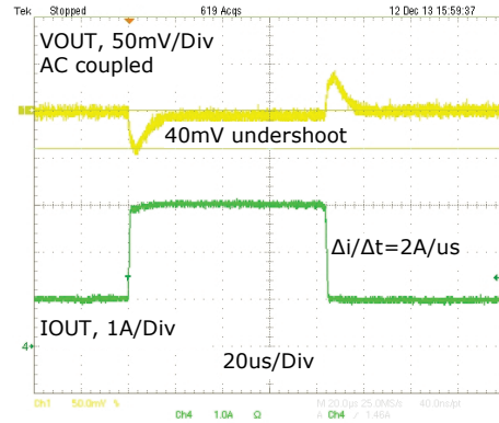
Fig. 7: Transient response, 1A-3A, 1.5VIN, 1VOUT
