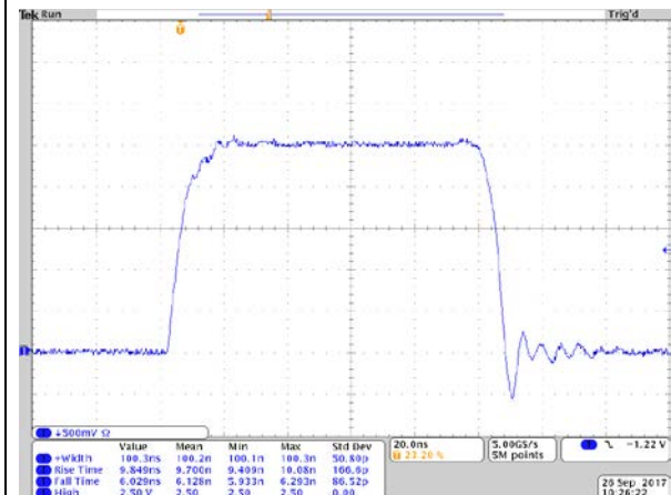
PCO-7121 (50 A, 100 ns, shorted load, inverted waveform)
