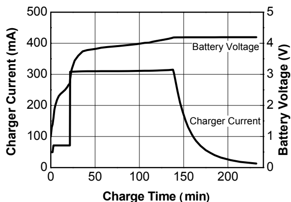
Figure 17. USB Charger Complete Charge Cycle V_{USB}=5.0\text{ V} , R_{IUSB}=6.52\text{ k}\Omega , 740 mA Battery, T_A=25^\circ\text{C}
