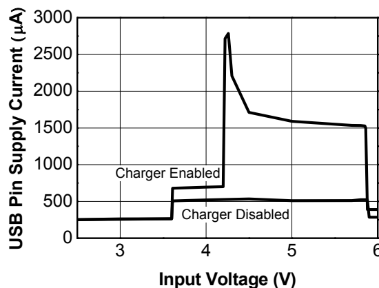
Figure 18. USB Pin Supply Current vs V_{USB} I_{BAT}=0\text{ mA} , T_A=25^\circ\text{C}
