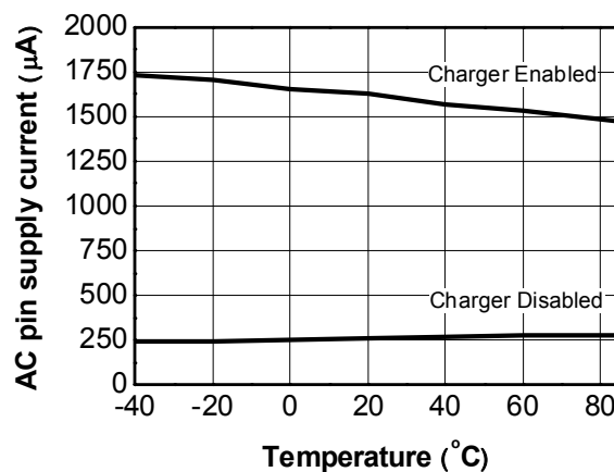
Figure 12. AC Pin Supply Current vs T_A V_{AC}=5.0\text{ V} , I_{BAT}=0\text{ mA}
