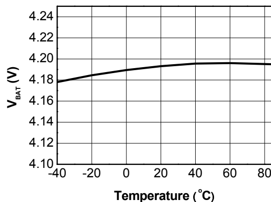
Figure 11. V_{BAT} vs T_A V_{AC}=5.0\text{ V} , I_{BAT}=0\text{ mA}
