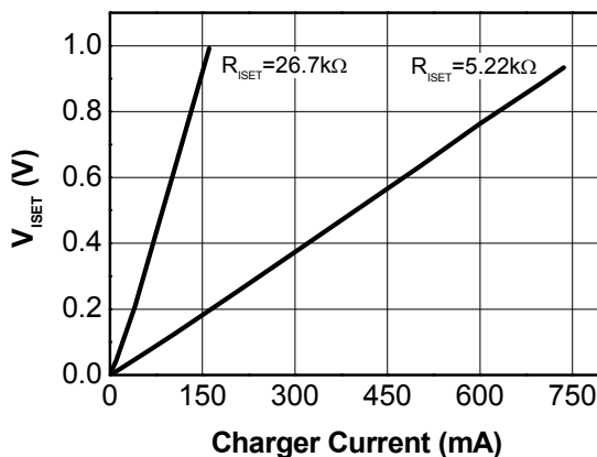
Figure 7. V_{ISET} vs AC Charger Charge Current V_{AC}=5.0\text{ V} , T_A=25^{\circ}\text{C}
