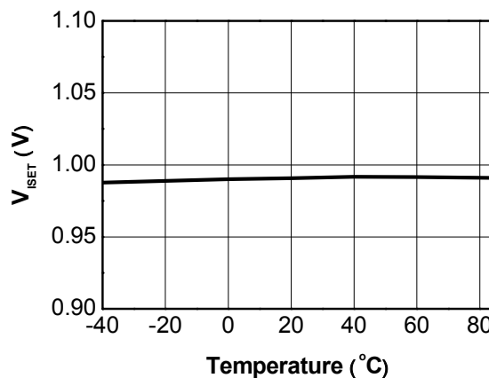
Figure 13. V_{ISET} vs T_A V_{AC}=5.0\text{ V} , R_{ISET}=5.22\text{ k}\Omega , V_{BAT}=3.7\text{ V}
