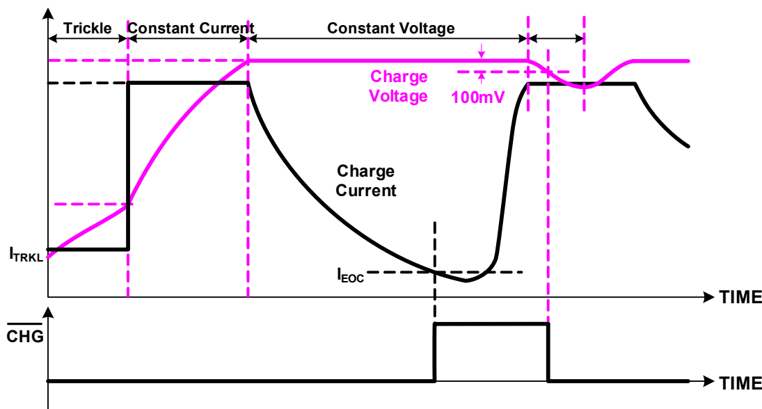
Figure 37. Typical Charge Cycle
