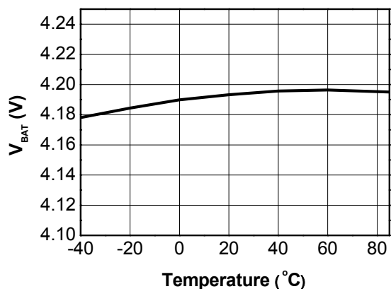
Figure 26. V BAT vs T A V USB =5.0 V, I BAT =0 mA
