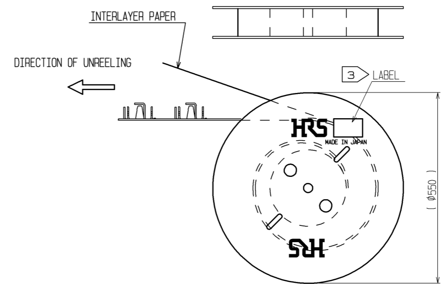
REEL STATE DRAWING(FREE)
