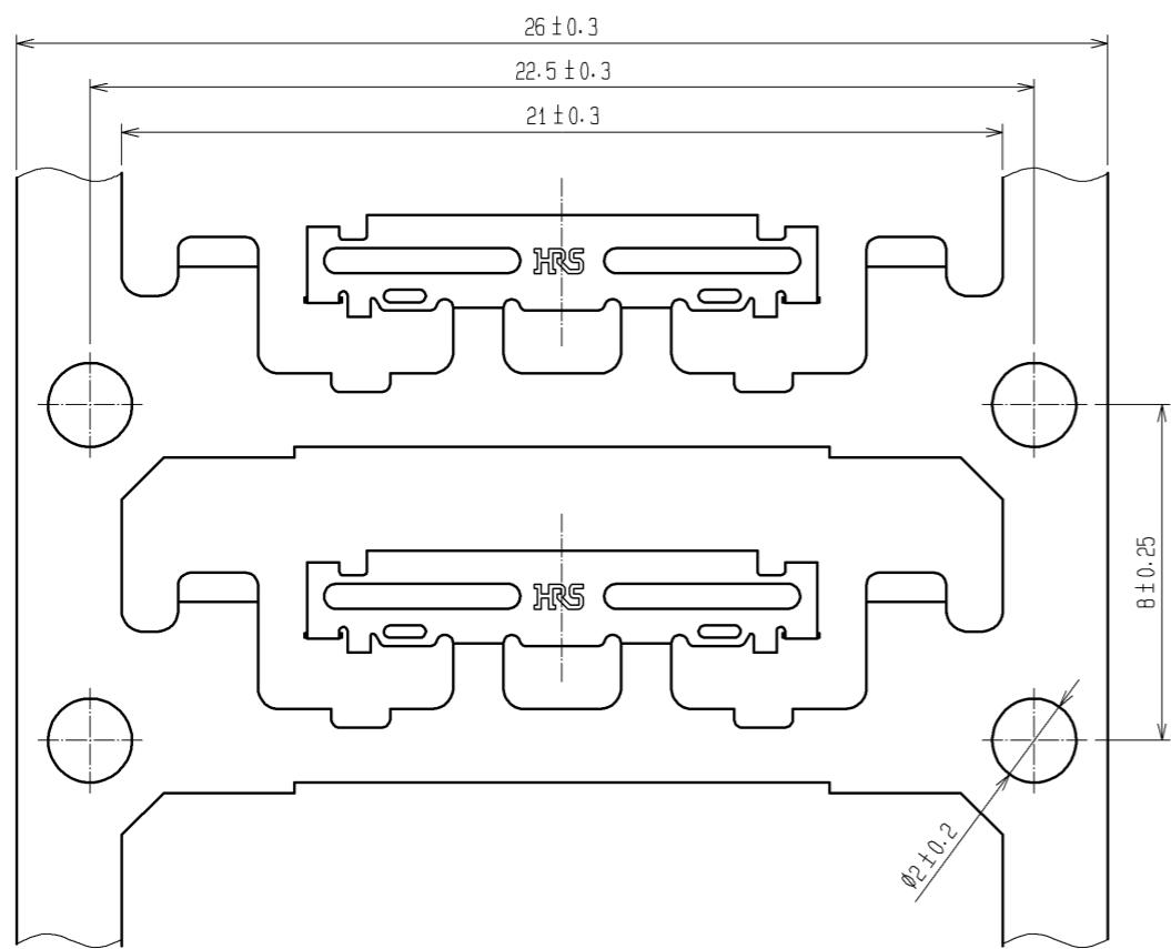
CARRIER STATE DRAWING(5:1)
